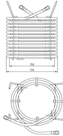
1serpentin/1 coil
